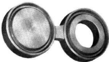
Spectacle Blinds (Figure 8 Blinds)
