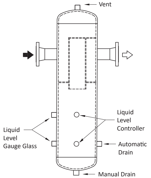
Type 110V-RV with Removable Vane
